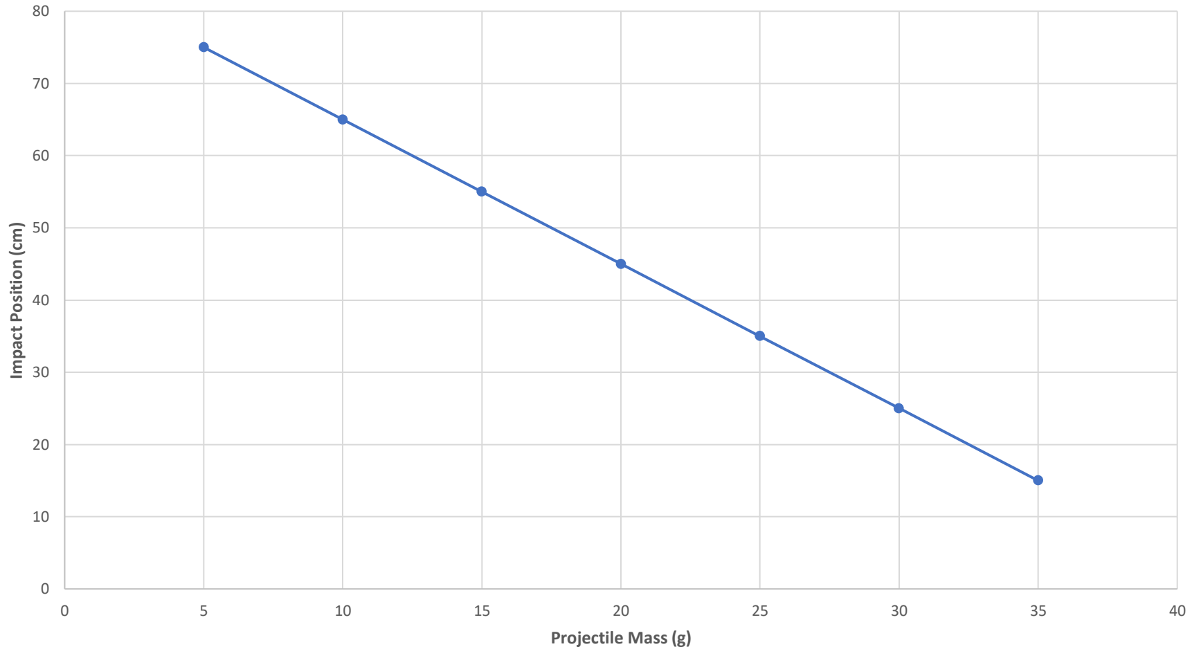
Impact Position vs. Projectile Mass
